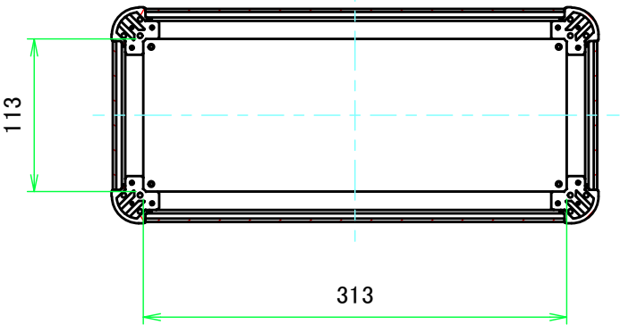
C-C (1:5)
